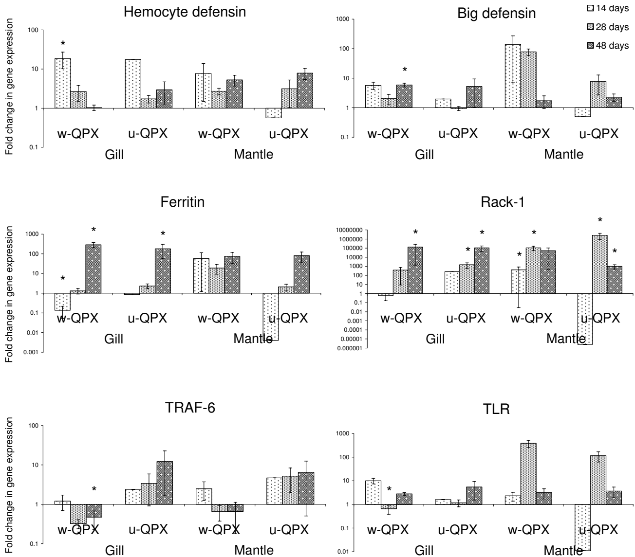
Figure 2 Relative expression by quantitative PCR of selected transcripts from SSH (hemocyte and big defensins, ferritin, RACK-1) and hemocyte (TRAF-6 and TLR) libraries. Expression levels were normalized to 18S RNA and presented as relative expression to controls (mean ± SD, n = 8 clams). * indicates significant differences of gene expression compared to controls at p < 0.05 (Student's t-test).
